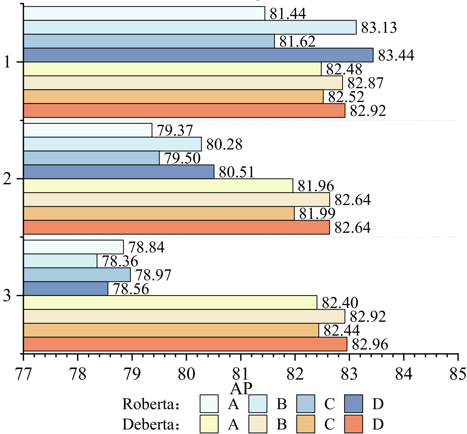
AP based on OPT generated text
